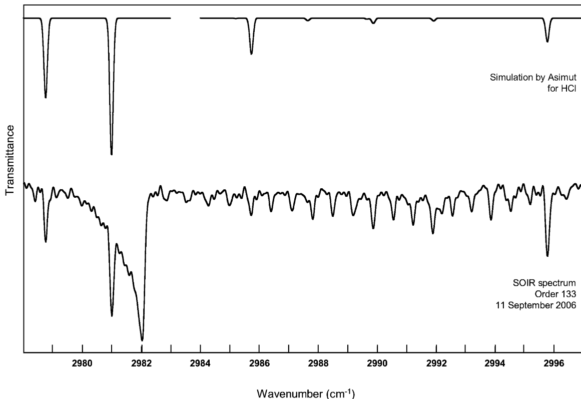
Fig. 2. One observed transmission spectrum taken around 83 km (lower curve) is compared to a synthetic spectrum of the absorption of HCl (upper curve). The main HCl absorption lines (including contributions from adjacent orders) are clearly identified in the observed spectrum. When corrected from these HCl absorptions, the main feature in the observed spectrum is even more resembling a Q branch, identified as the 628 isotopologue of CO 2 .
