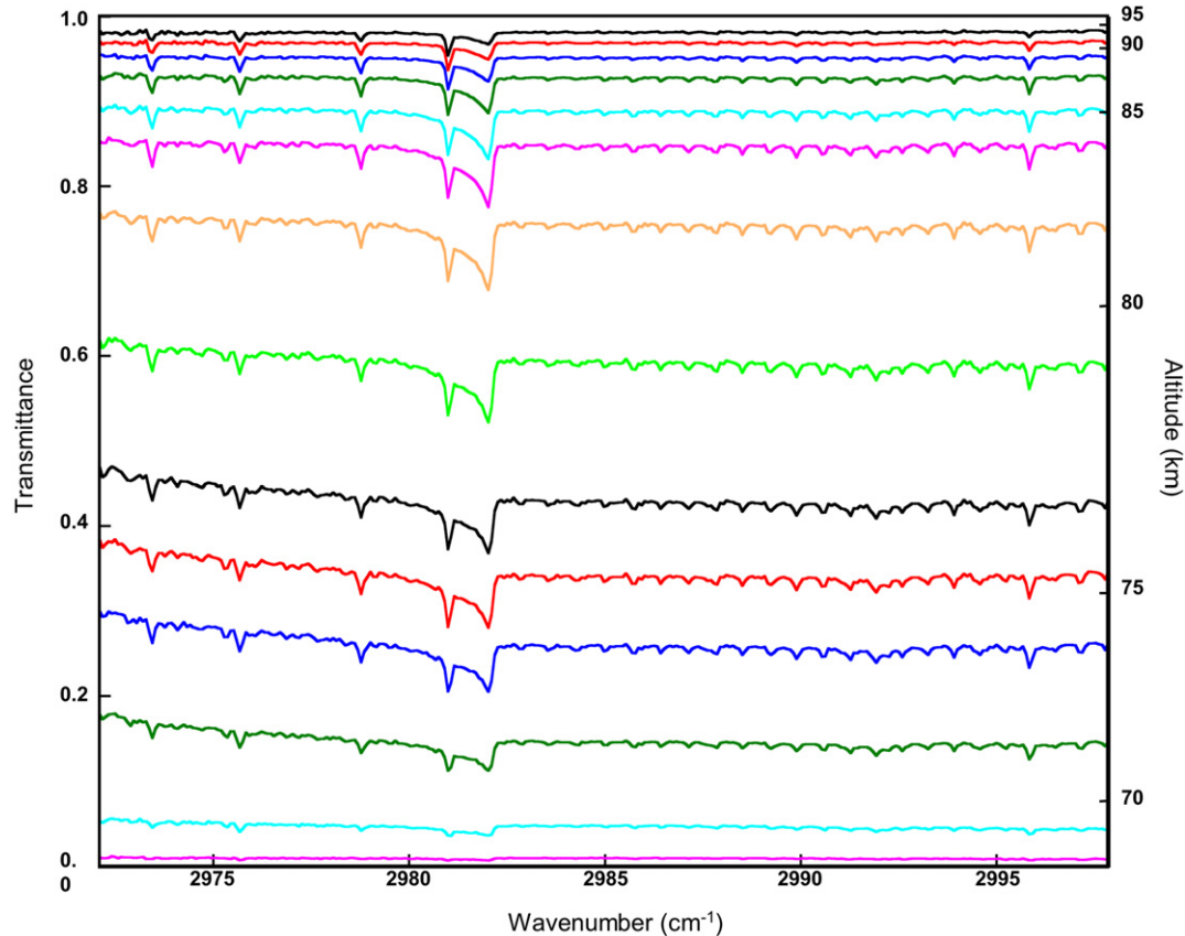
Fig. 1. Atmospheric transmission measured by SOIR during one single occultation. There is one different curve acquired each second, and the corresponding tangent altitude is indicated on the right scale (non-linear, not regular). Each transmission spectrum is obtained by ratioing the solar spectrum seen through the atmosphere to a reference spectrum obtained outside the atmosphere. The overall transmission is decreasing with altitude, owing to the continuous absorption by aerosols above the main cloud deck (the so-called haze). The main spectral feature at 2980\text{--}2982\text{ cm}^{-1} looks like an unresolved Q branch. The depths of all lines (relative to the continuum) are increasing with decreasing altitudes and increase of the slant optical path.
